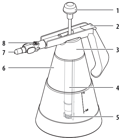
Fig. 1: Parts of the special pressure sprayer
